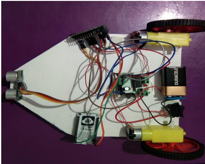
Figure.11 Initial stage of Implementation prototype
