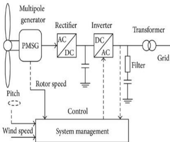
Fig(4) Structural Architecture of WCS
