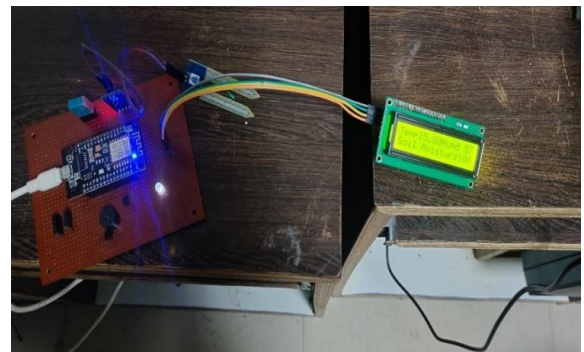
Fig. 7. DHT 11 testing.
