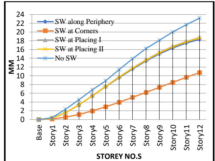
Fig.11. Storey Displacement
