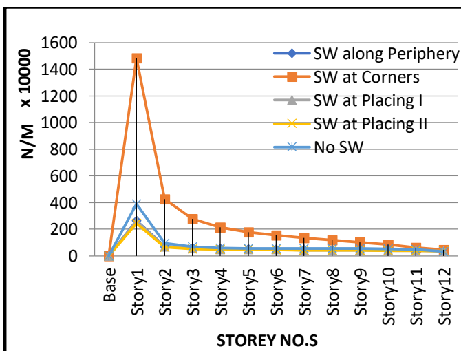
Fig.14. Storey Stiffness
