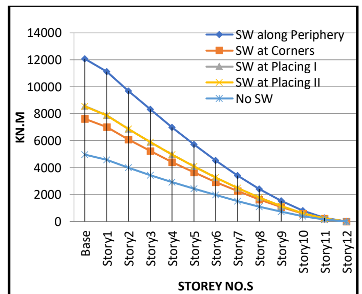
Fig.16. Overturning Moments
