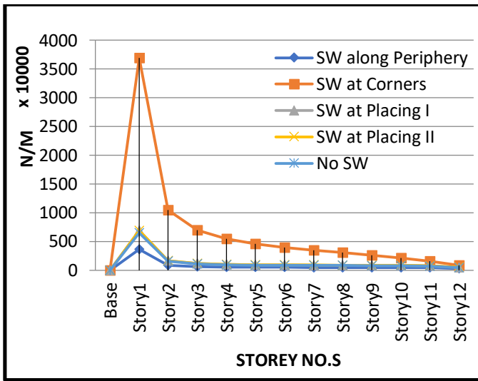
Fig.13. Storey Stiffness
