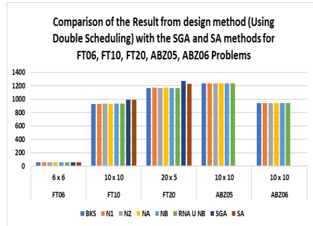
Fig 4 Comparison of the result from design method (using double scheduling)
