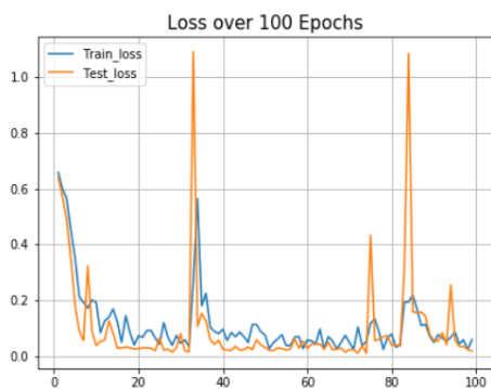
Figure 1.3. Accuracy-Loss Graph
