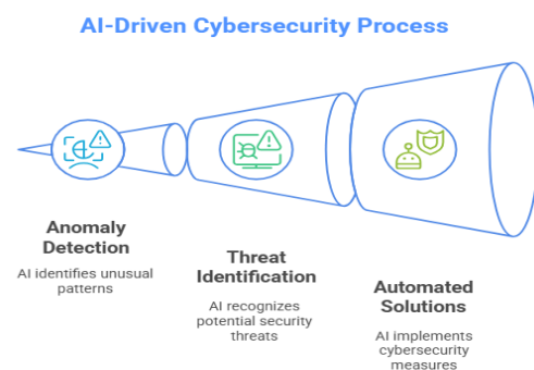
Figure 1: AI-driven cybersecurity
