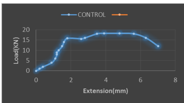
Figure 1 Figure 1: The Load – Extension Graph of the As-Cast Low Carbon Steel
