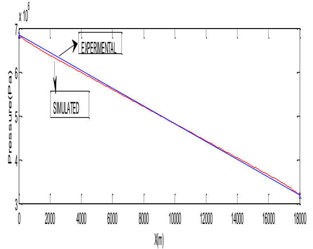
Figure 3: Comparison of simulated pressure distribution along the length of the pipeline with Shell data
