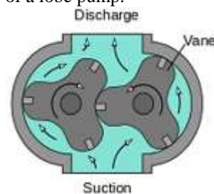
Figure 8 the Internal Parts of a Lobe Pump
