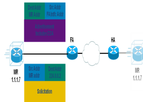
Fig.3. Mobile Router Advertisement
