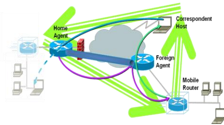
Fig.6. Triangle routing
