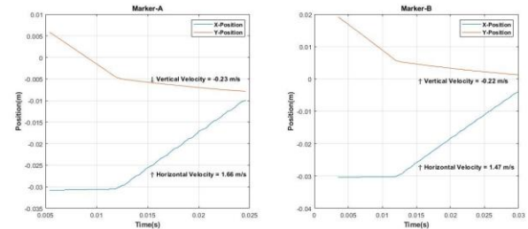
Fig. 10: Displacement plot of 2 markers on rod-2 impacting at 30 degrees
