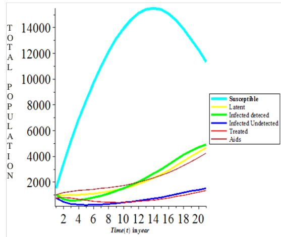
Figure 1: Plots of Total Population against time t for various value of \beta (0.3)
