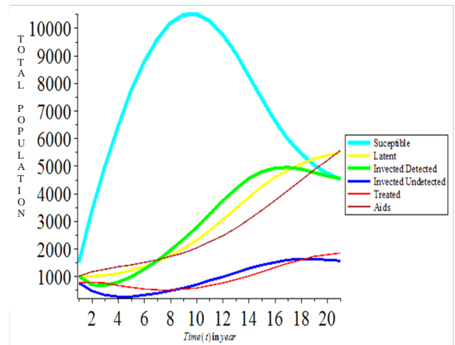
Figure 2: Plots of Total Population against time t for various value of \beta (0.5)
