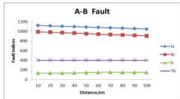
Fig.11 Variation of fault indices with distance at a constant Fault inception angle 100^{\circ} from terminal-1 for A-B fault
