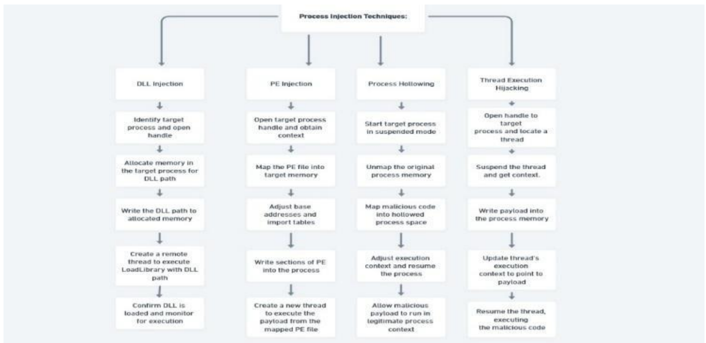
Fig.1.Process Injection Techniques
