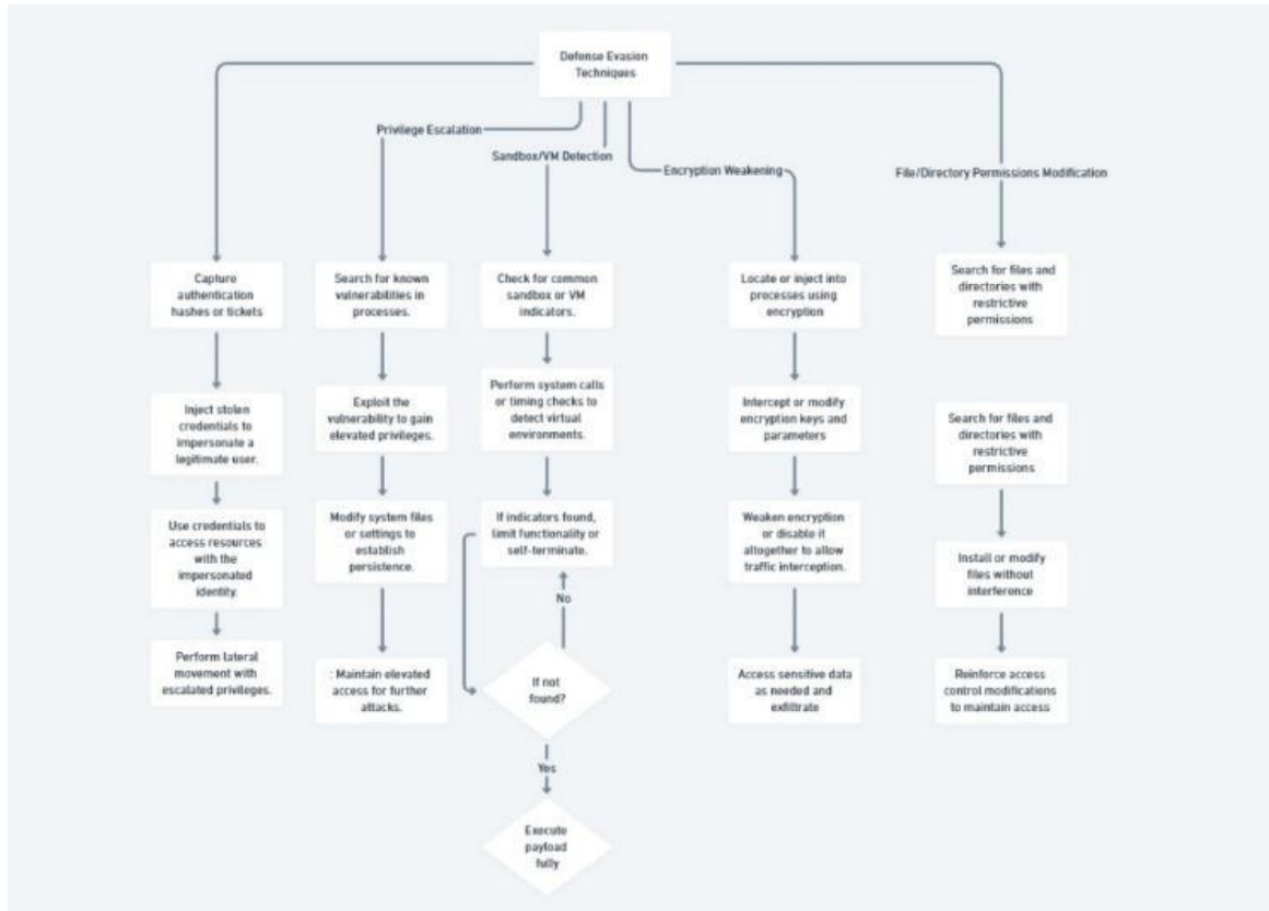
Fig.3. Defense Evasion Techniques
