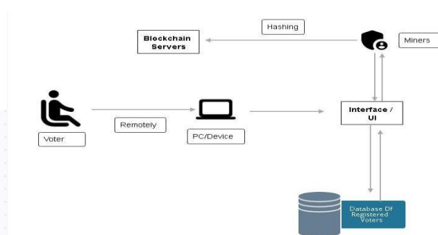
Figure 2: E-voting Flow
