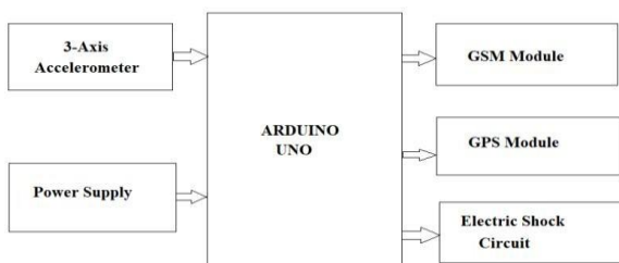
Fig.1 Block Diagram
