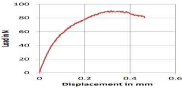
Fig.4.7 Typical Load-Displacement diagram of miniature specimen in transverse direction (experimental)
