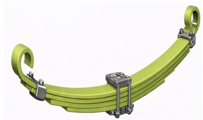
Figure 5: Final composite mono leaf spring with reinforced eye ends and mounting arrangement.
