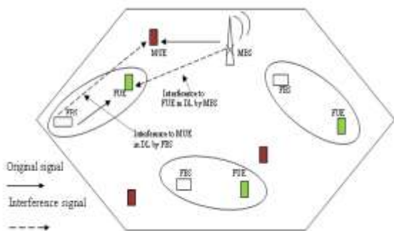
Fig 3 Cross-Tier Interference
