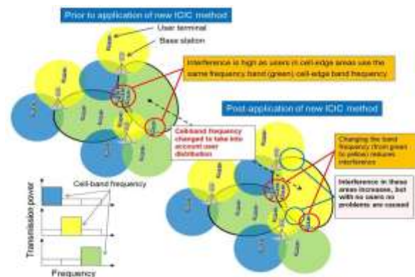
Figure 4: ICIC technique
