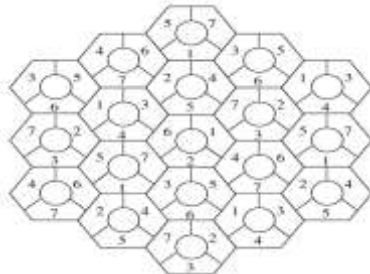
Fig 7. Frequency Reuse of Alcatel's Proposal
