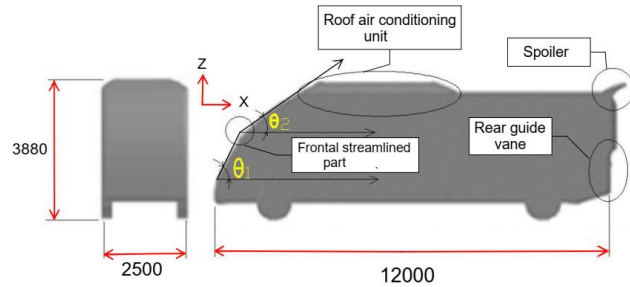
Figure.3: Streamline design concept used.
