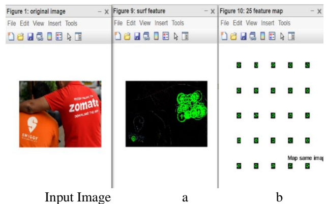
Fig.5 SURF feature
