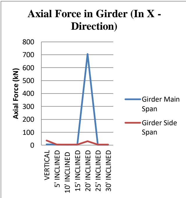
Chart 3. Axial Force in Girder X - Direction
