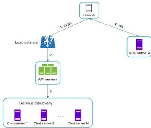
Fig 1: Proposed Architecture
