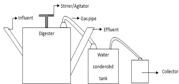
Fig 1: Digester
