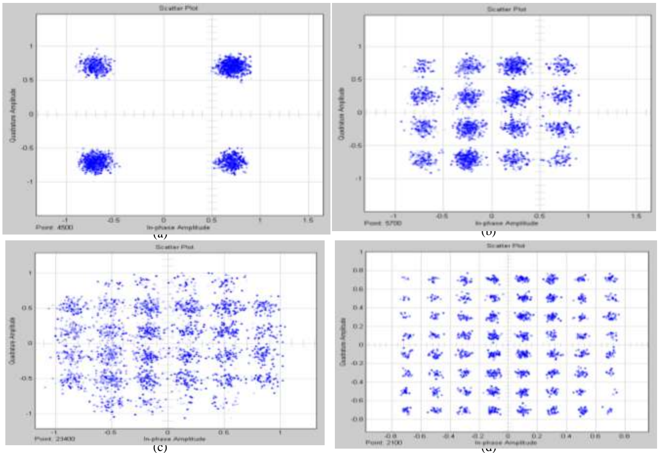
Fig. 7. The constellation diagram for M-QAM (a) 4-QAM, Eb/No=20 (b) 16-QAM, Eb/No=20 (c) 32-QAM, Eb/No=20 (d) 64-QAM, Eb/No=30
