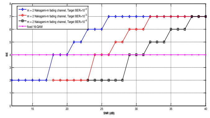
Fig.18. SE versus SNR for adaptive modulation under m=2 Nakagami- m fading channel for different BER target
