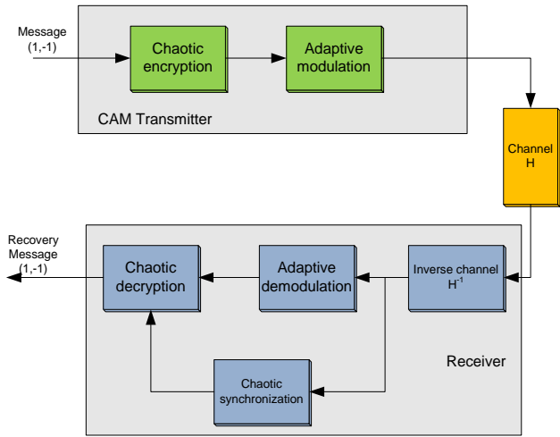
Fig. 1. Simple block diagram for CAM system
