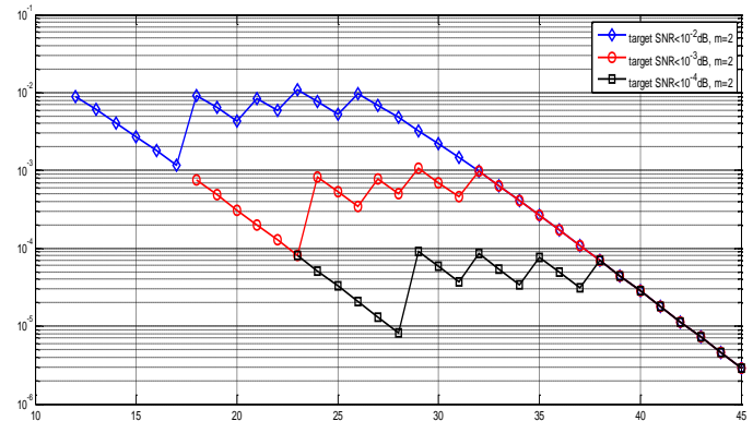
Fig.16. BER versus SNR for adaptive modulation under m=2 Nakagami- m fading channel for different BER target
