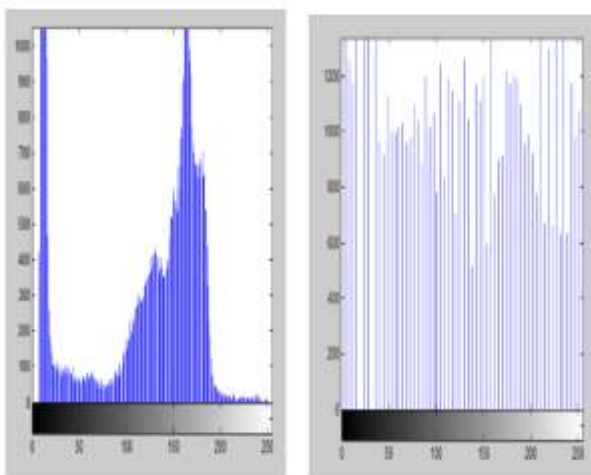
Fig 4.4(b) Histogram of Original and Equalized Image
