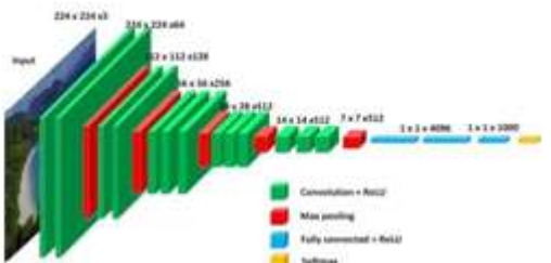
Figure 4 – VGG Model [17]
