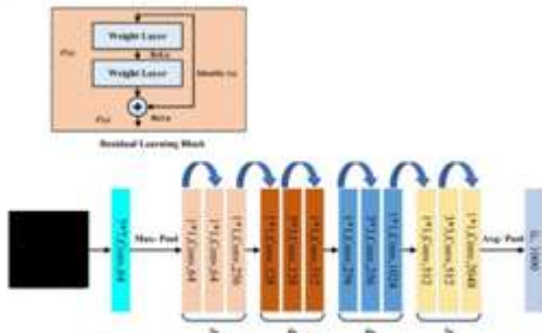
Figure 3 – RESNET Model [8]
