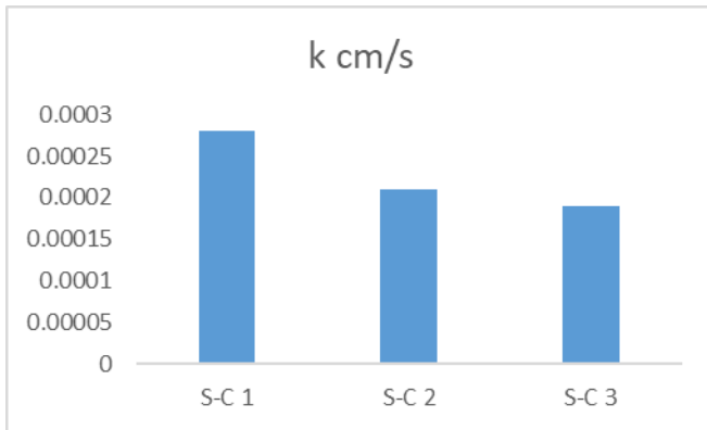
Fig. 2. Permeability of cement-sand mixtures
