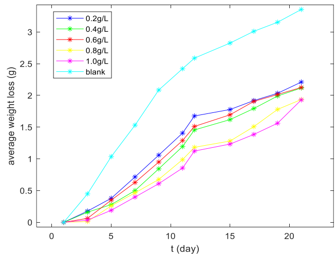
Fig. 1: Average weight loss of coupons against time at different concentrations of extract
