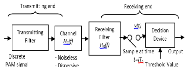
Fig. 1 Baseband Binary Data Transmission System
