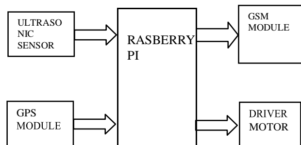
Figure 2: Block Diagram
