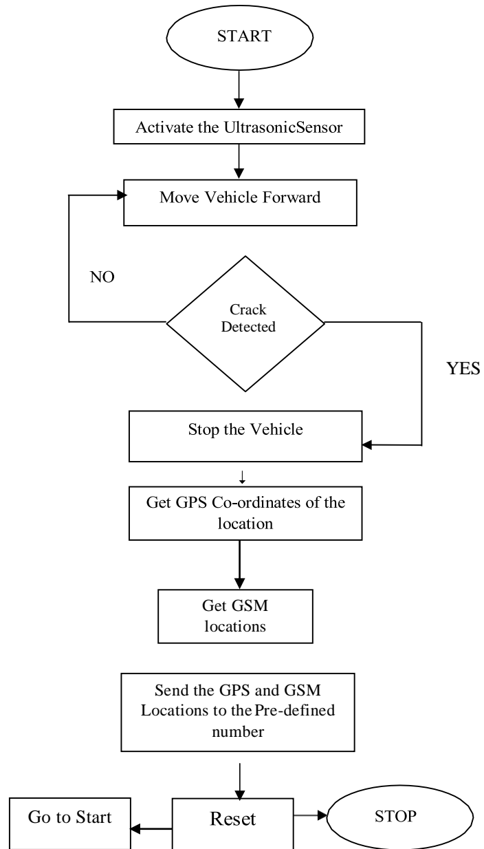
Figure 3: Program Algorithm
