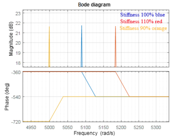
Fig. (9): The enlargement of the fourth mode of the Bode diagram in Fig. (7)
