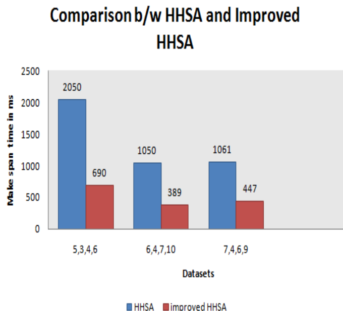
Fig. 6. Compariosn for HHSA and Improved HHSA
