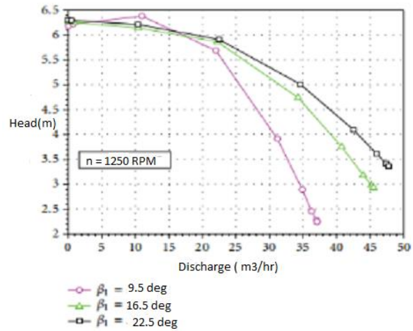
Figure 7: The graph of total head as verses flow rate (discharge) , studying the non cavitating performance.
