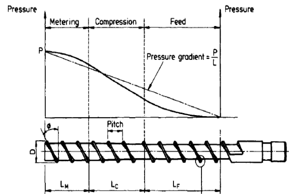
Fig.1. Screw Zones [6]
