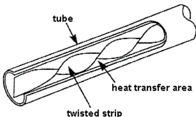
Fig. 3 Twisted Tapes.
