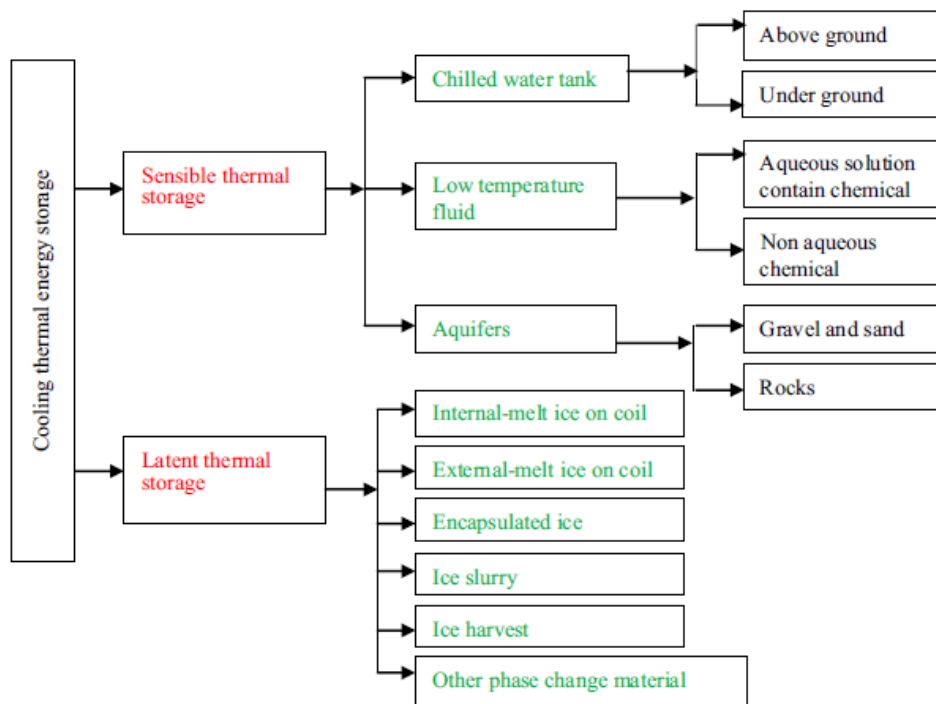
Fig.3. Classification of Cooling Thermal Energy Storage [14]
