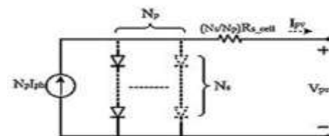
Fig. 1. Multi-diode model
