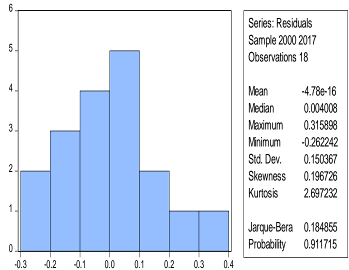
Graph 1: Normal Probability Distribution graph of residuals
