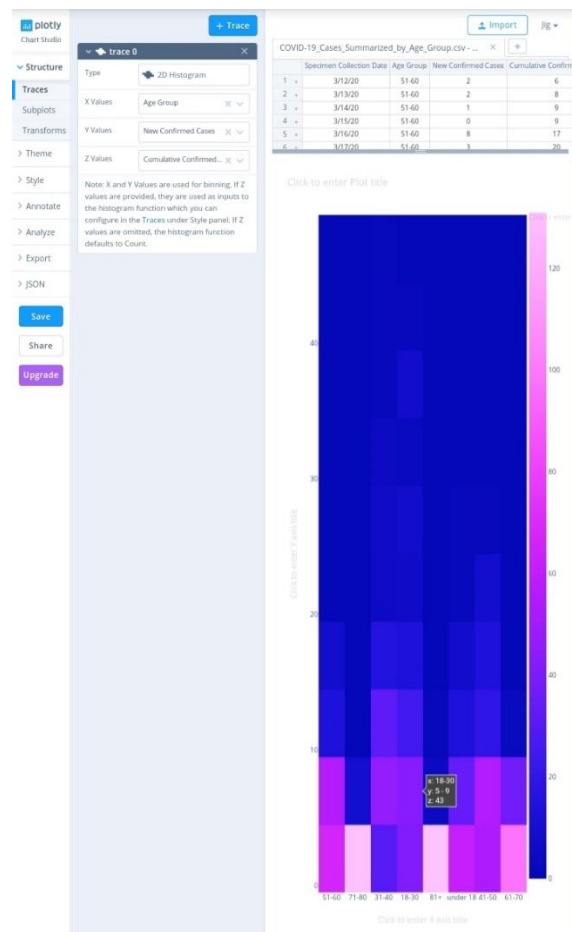
Figure 2 : 2D Histogram
