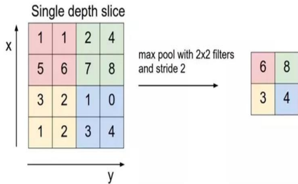
Fig 8: Max Pooling [8]
