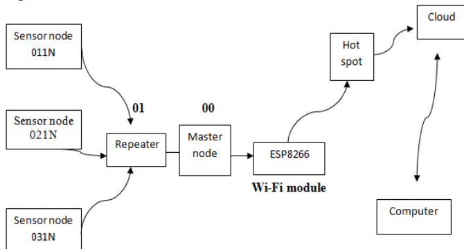
Figure 1:- Block Representation of Sensor Node
