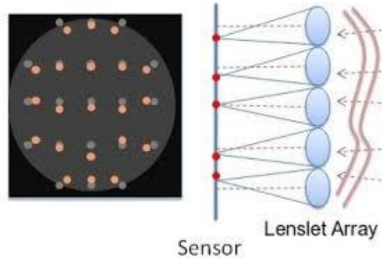
Fig 13: SHWFS simulation 15
