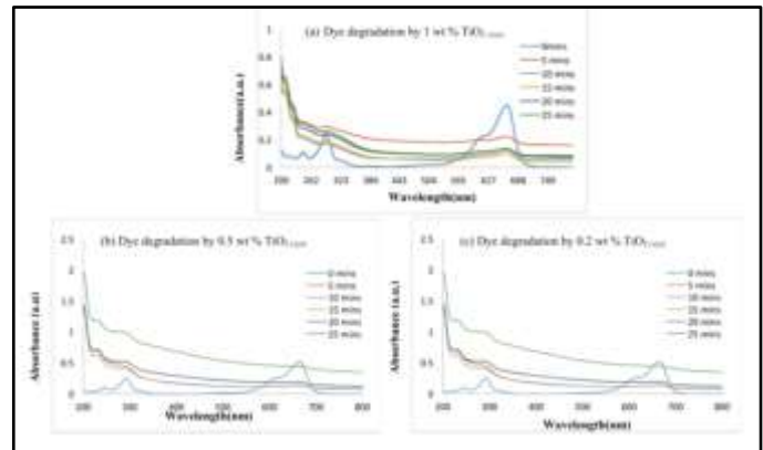
Fig. 9. Dye Degradation by (a) 1 wt % Ag/TiO 2cryst , (b) 0.5 wt % Ag/TiO 2cryst and (c) 0.2 wt % Ag/TiO 2cryst .
