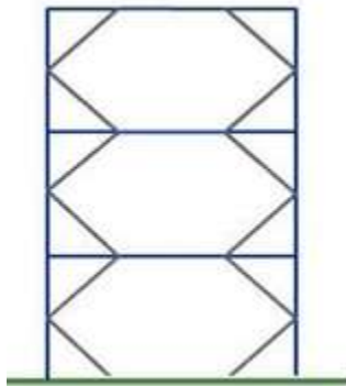
Fig 2.4 K-bracing
