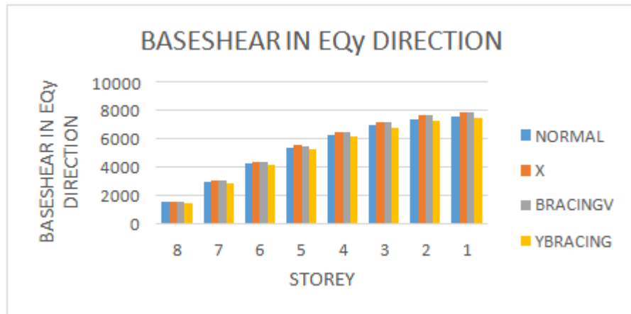
Graph 4.12 Base Shear in EQy direction for Sand
