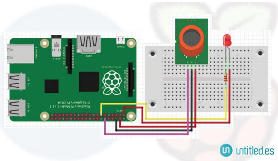
Fig 2.8.2: Connection Configuration [1]
