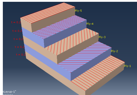
Fig. 7 (b) Laminate stacking sequence in non-circular tube
