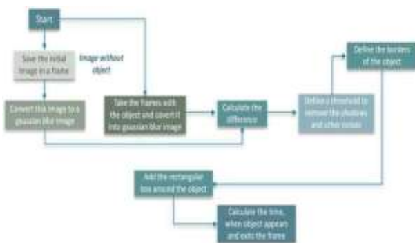
Figure 4. Flow Diagram
