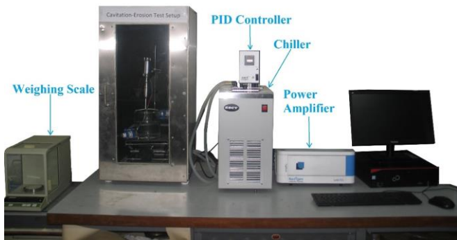
Fig. 2. Vibratory Cavitation erosion Test Setup
